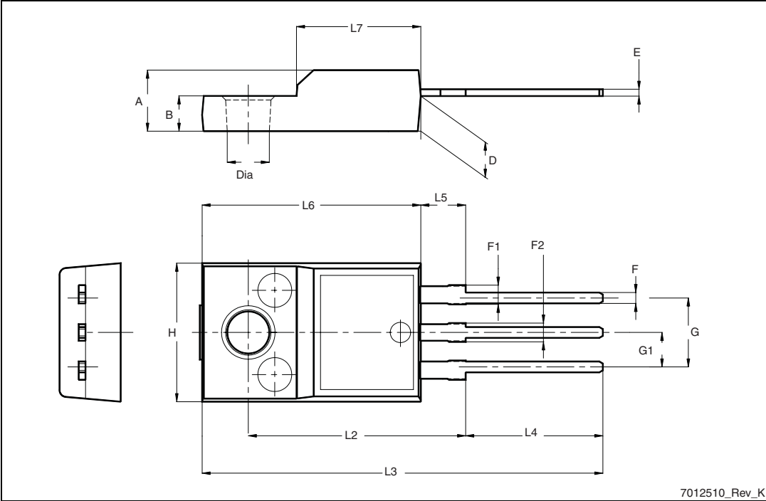
Figure 22. TO-220FP drawing
